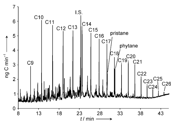
Figure 4. Mass-flow chromatogram of a diesel-fuel sample.
